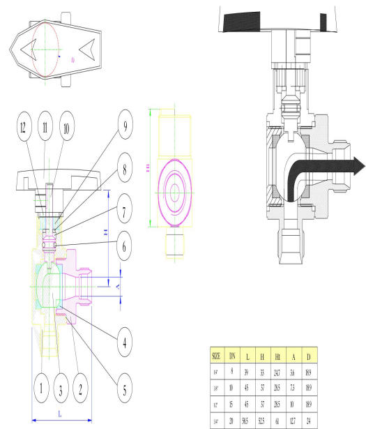
Angle valve
