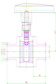
Tri clamp end valve
