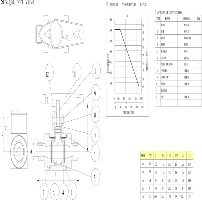
Straight port valve
