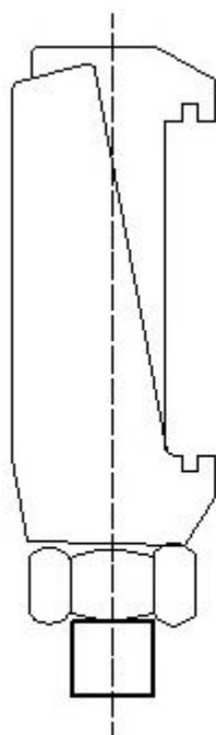
I022-ISO double claw clamp-steel(zinc plated)
