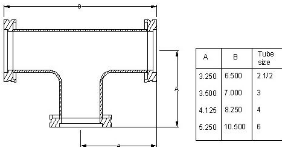
I021-ISO Tee
