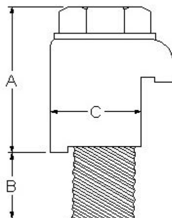
1008-ISO single claw clamp
