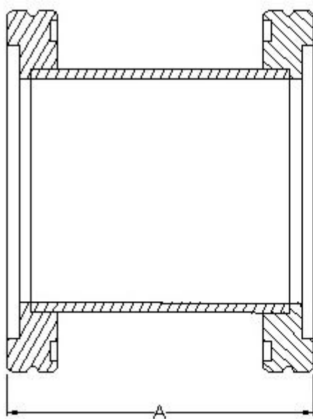
I011-ISO full nipples
