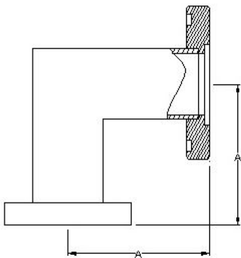
I014-ISO 90° elbow mitered
