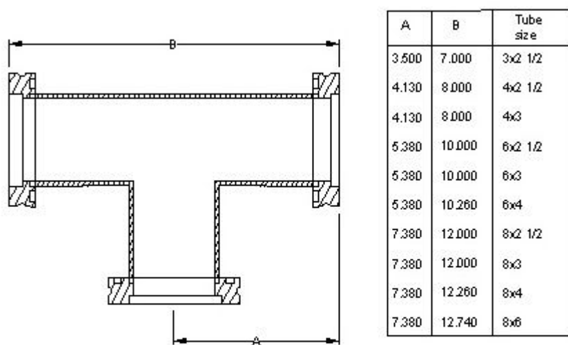
1020-ISO reducing tee
